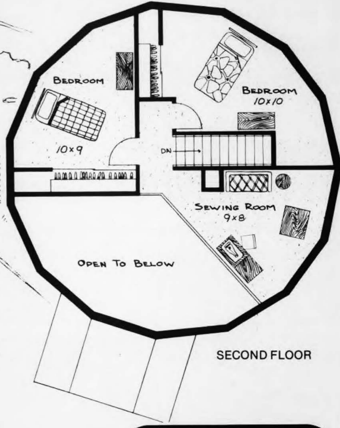
METCALFE RESIDENCE Northwestern Wisc. 10 meter (33') 5/9 Dome
