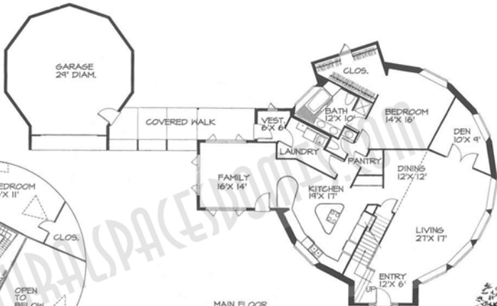
MAIN FLOOR 2,250 SQ. FT.
