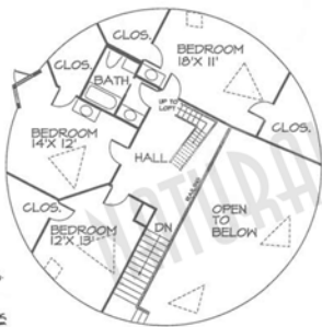
UPPER FLOOR 1,100 SQ. FT.
