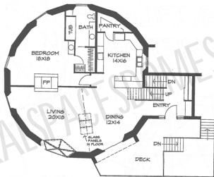
MAIN FLOOR 18'15" SQ. FT.
